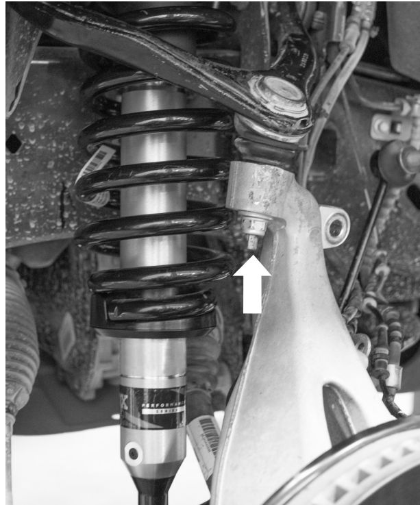
Fig. 15: Reattach the UCA to the upright.
