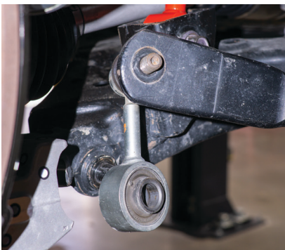
Fig. 2: Sway bar end link.
